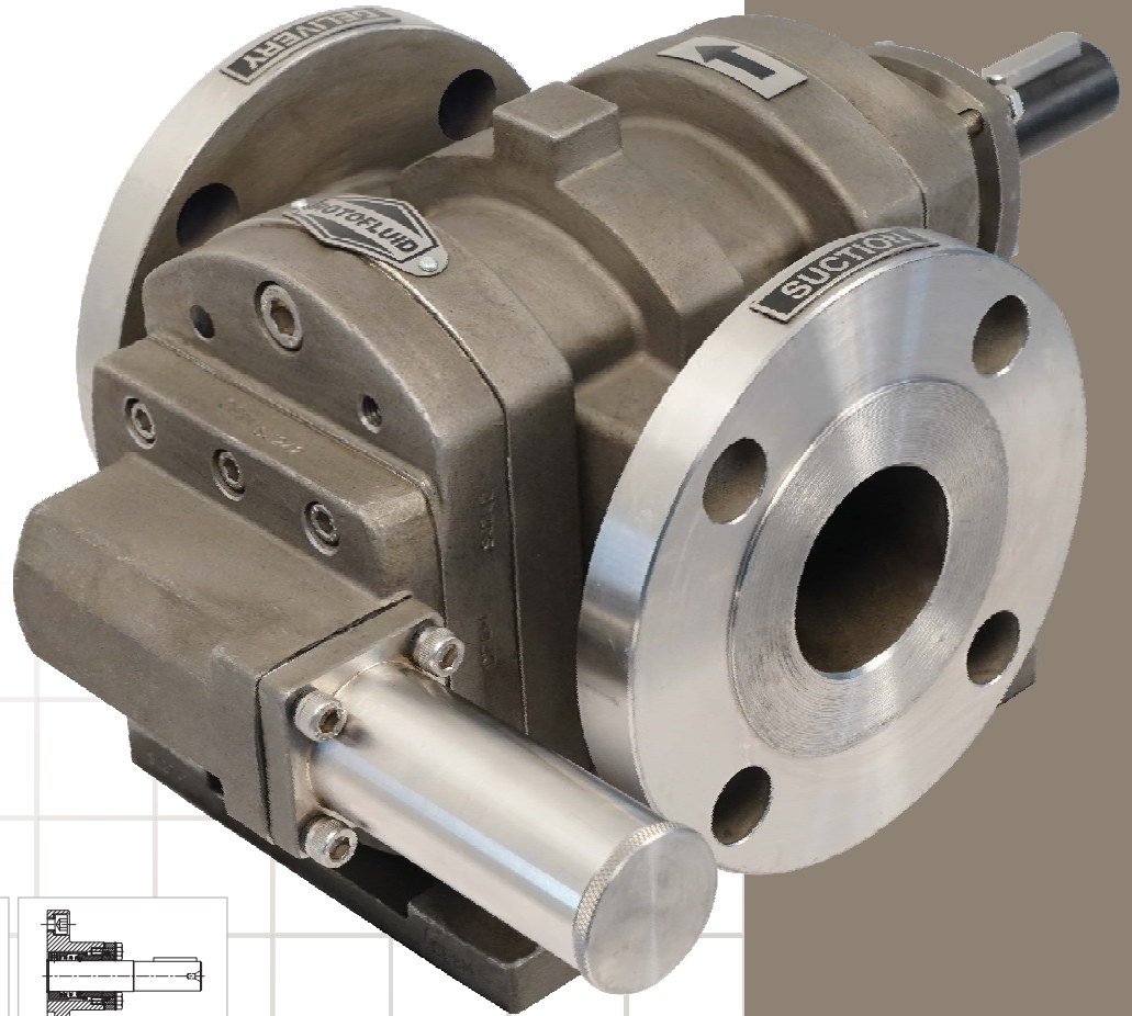
MECH. SEAL IN STUFFING BOX
