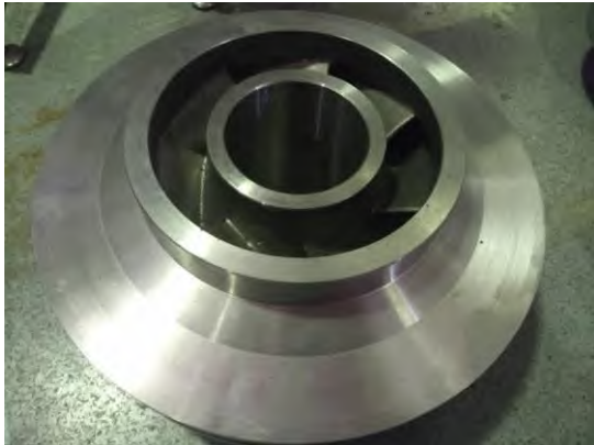
Duplex investment casting-400 mm Q=500 m 3 /hr H=600 m (4 stages)
