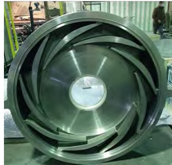
Duplex Investment and Sand Casting 320 m 3 /hr – 60 bar
